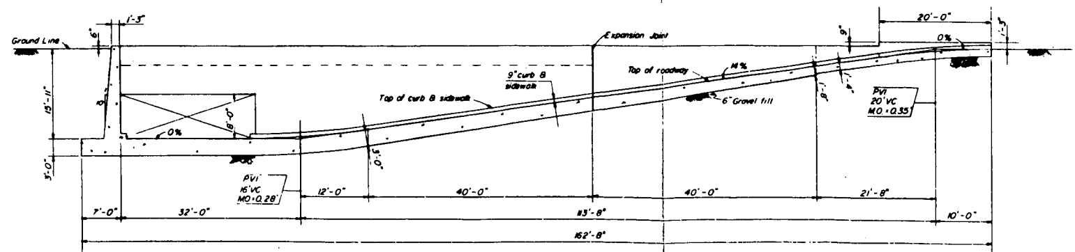
Fig. 4—Parking garage—shelter underground test section.
